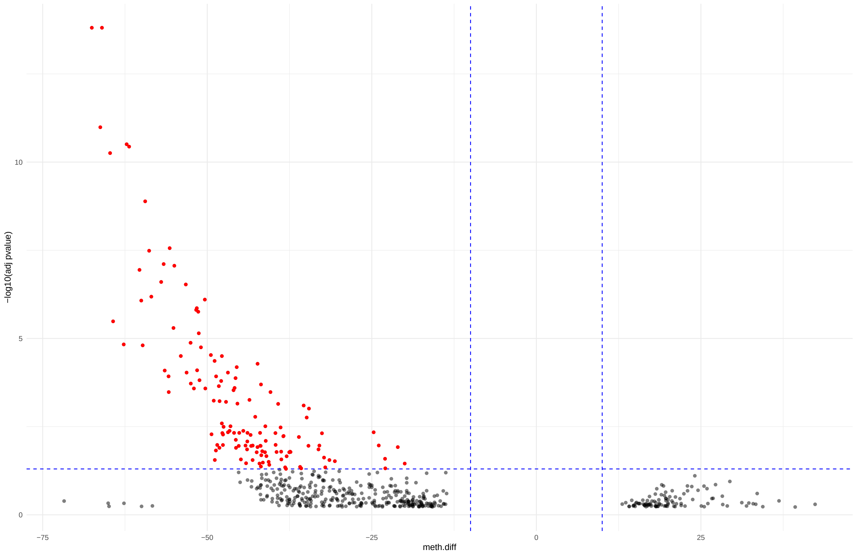
Volcano plot: infection
