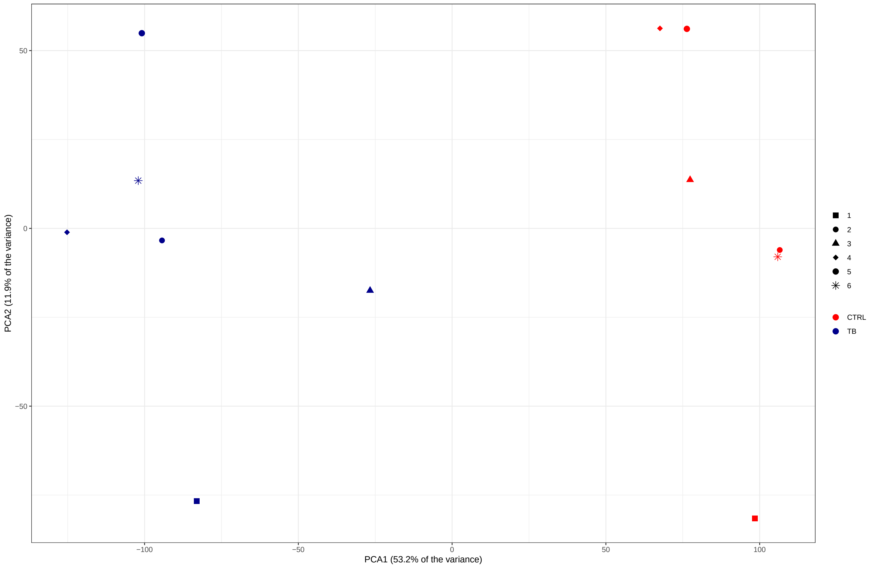
Explorative analysis – PCA
